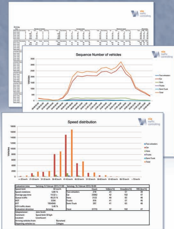
Sample evaluation of a viacount traffic counter.
